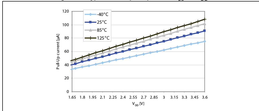
Figure 31. Typical NRST pull-up current I_{DU} vs. V_{DD}
