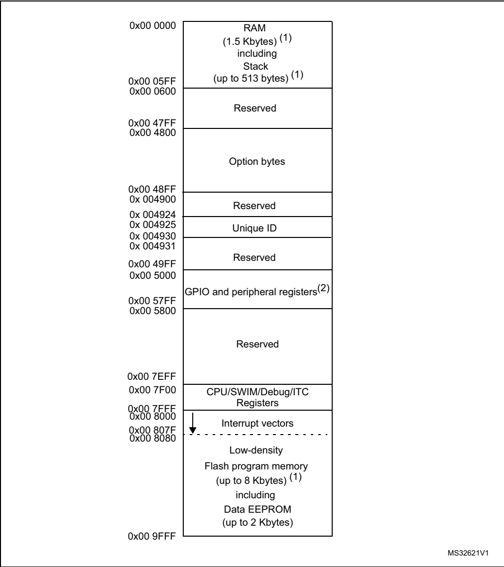
Figure 8. Memory map
