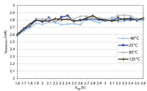
Figure 12. I_{DD(RUN)} vs. V_{DD} , f_{CPU} = 16 \text{ MHz}
